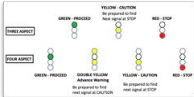
MULTI ASPECT Colour Light Signals
